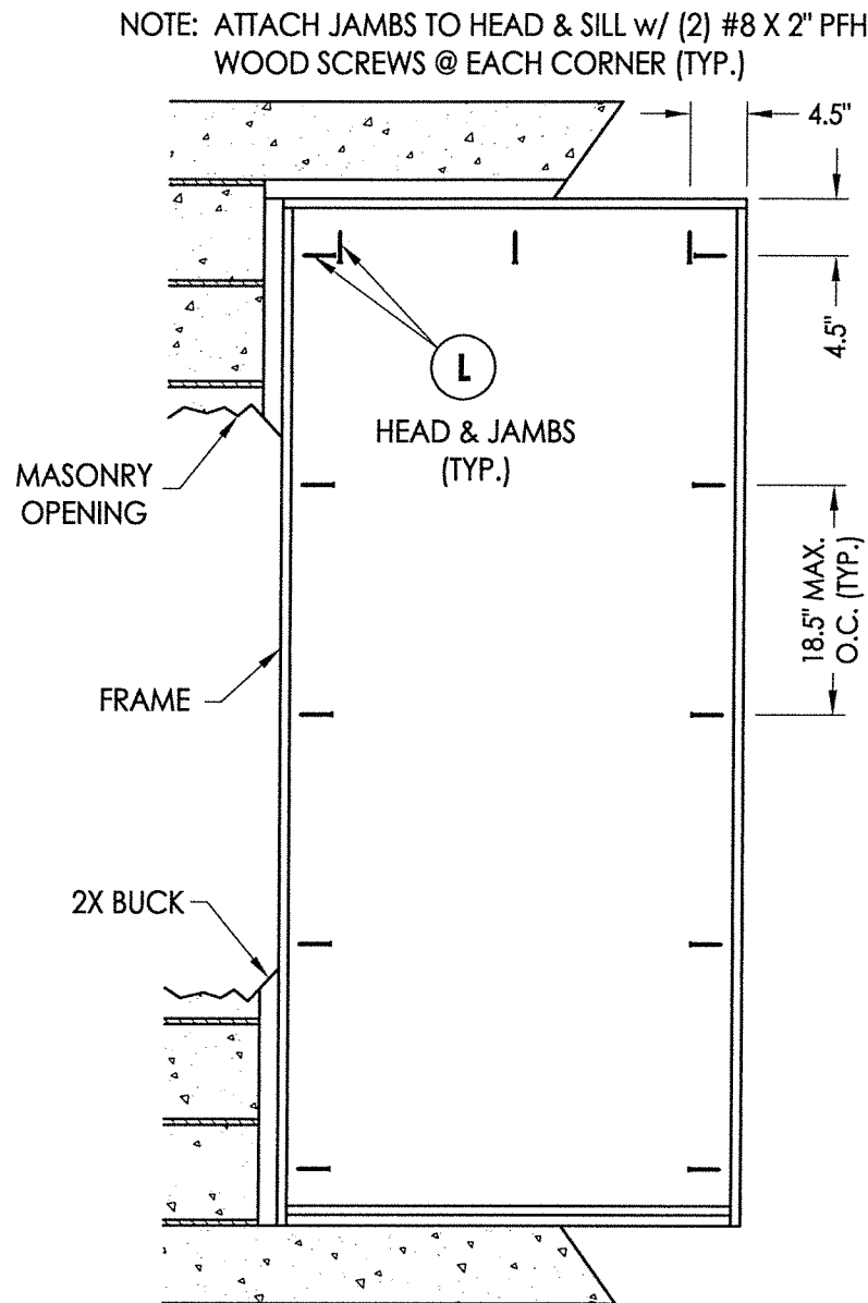
FRAME ANCHORING Masonry 2X buck construction
