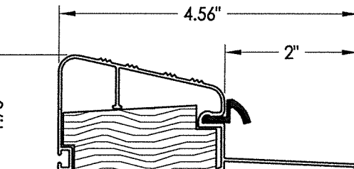
32 OUTSWING HIGH DAM BUMP THRESHOLD DLP (QOSR)
