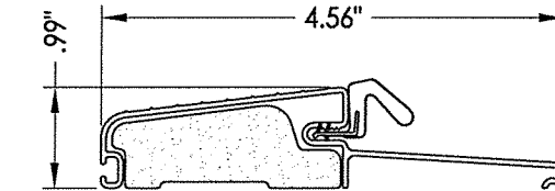
31 OUTSWING BUMP THRESHOLD Endura (FOB4566AA)
