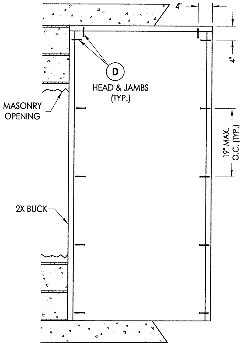
BUCK ANCHORING
