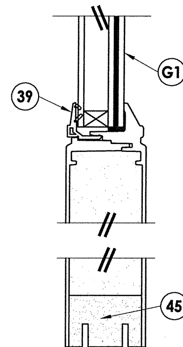
2 VERTICAL CROSS SECTION
