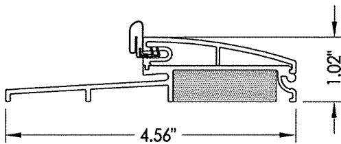
34 OUTSWING BASE SILL w/ BUMPER THRESHOLD CAP
