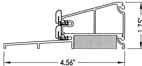
35 OUTSWING BASE SILL w/ BUMPER THRESHOLD HIGH DAM CAP
